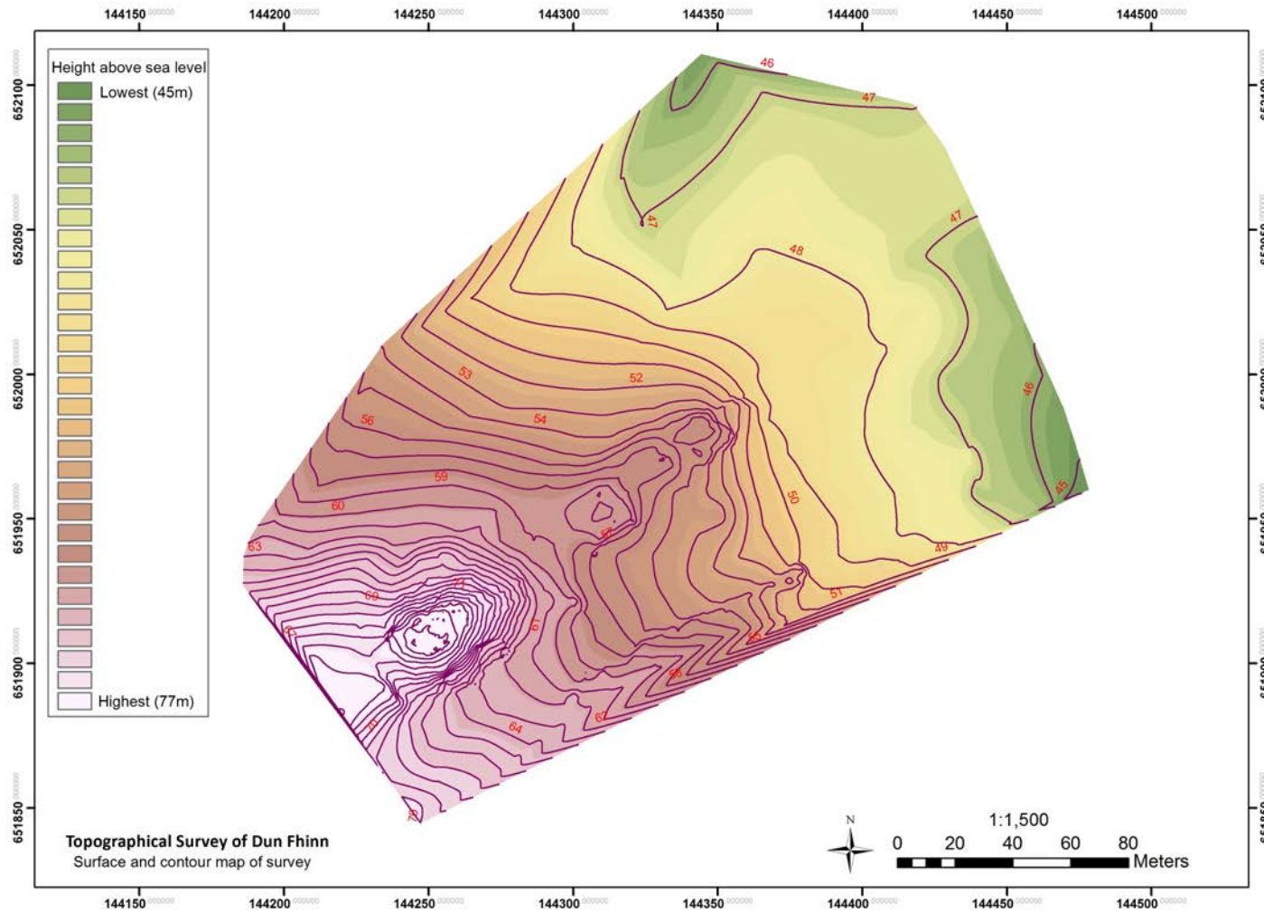
Figure 5: Topographical survey of Dun Fhinn and surrounding area
